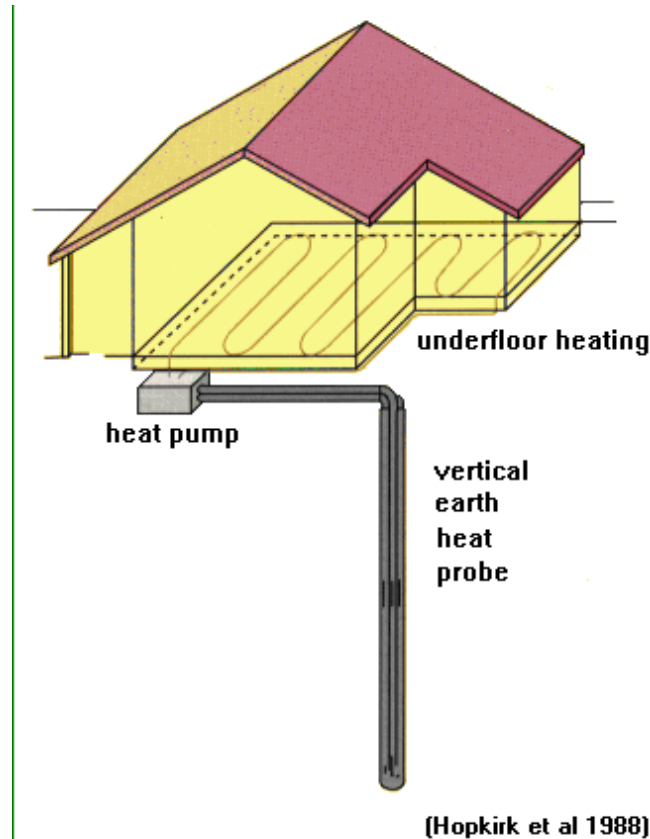
Schema of a U tube system installed
